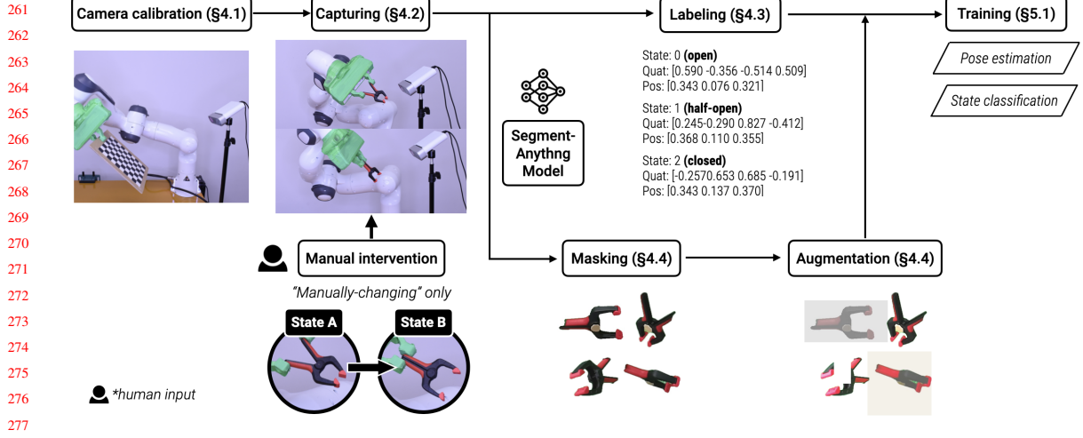
Fig. 4. Overview of RoCap. RoCap pipeline consists of camera calibration (§4.1), data capturing (§4.2), data labeling (§4.3), data processing (§4.4) and data augmentation (§4.4). By training on an existing deep learning framework, RoCap achieves object segmentation, state classification and pose estimation for appearance-changing objects.
