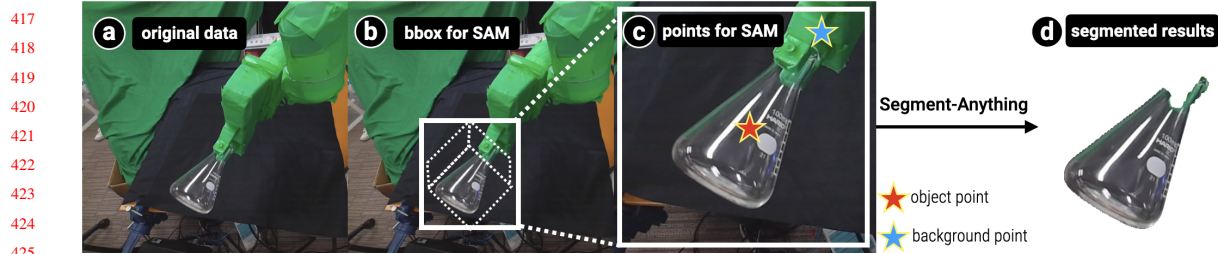
Fig. 8. Data processing of data collected in by RoCap. RoCap generates mask for each image (d) by prompting SAM with bounding box (b) and points (c).
