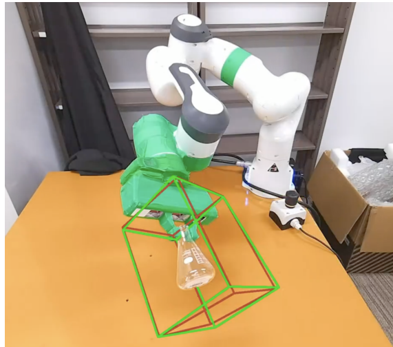
Fig. 9. Quantitative evaluation setup. The green bounding box represents the ground truth and the read bounding box represents the predicted pose.
