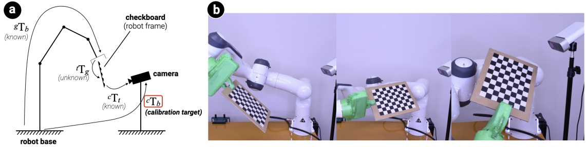
Fig. 5. Illustration of the eye-to-hand camera calibration (a). The robotic arm grip a checkerboard and move to multiple positions and orientations for an accurate calibration (b).
